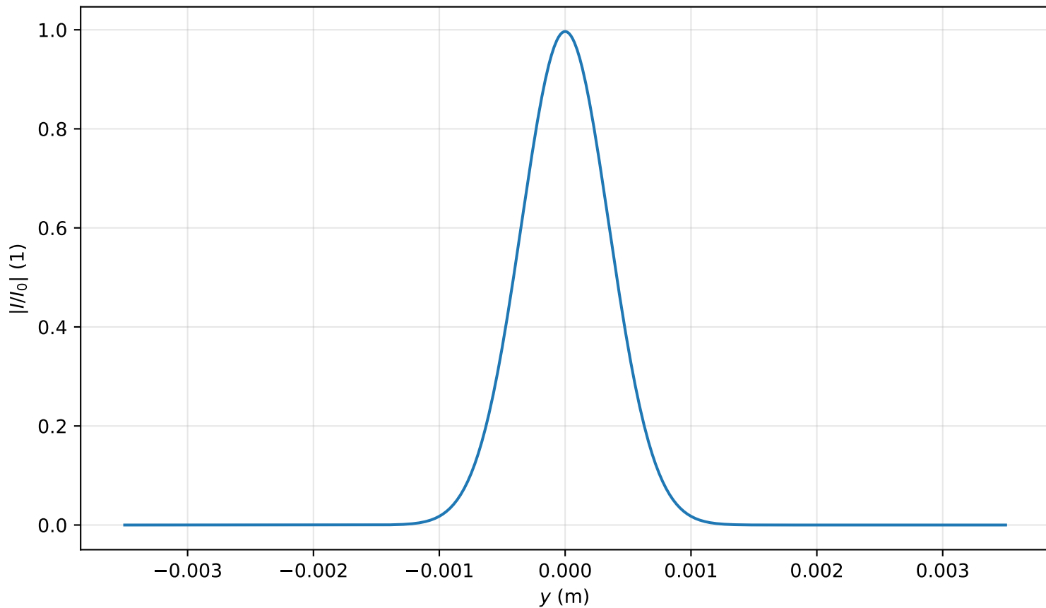
Intensity profile I(x=0, y, z=0.239)/I_0 , P_{in}=0.2P_{cr} , artificial time
